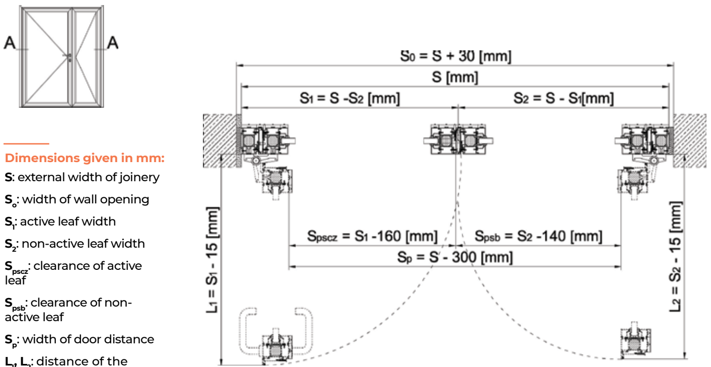
Figure 13. Horizontal cross-section of fire-resistant double leaf EI30 doors (similar to EI15, EI45 and EI60)
